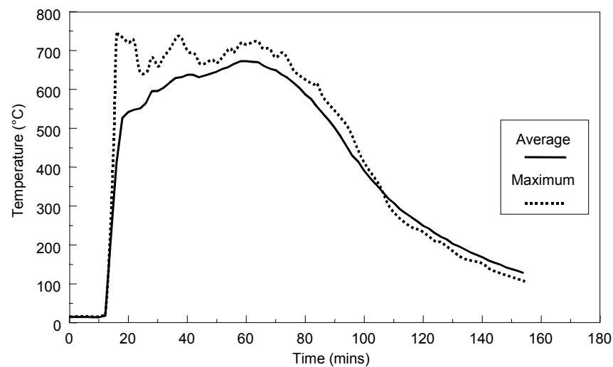
Figure 2.13 Maximum and average recorded atmosphere temperature
