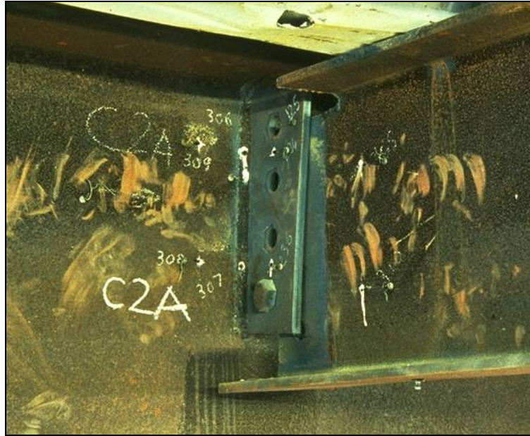
Figure 2.8 Fin-plate connection following test
