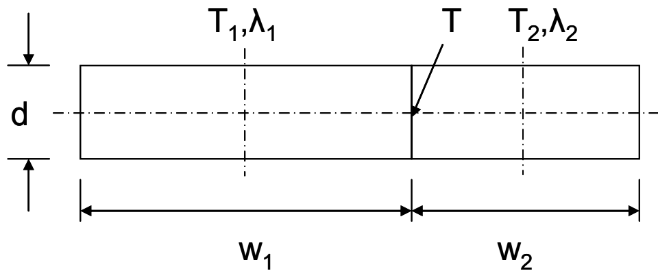
Figure 6.13 Basic conduction model
