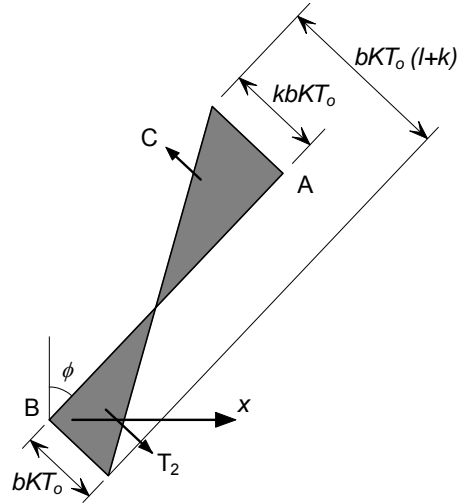
Figure 5.15 Forces applied to element 1, yield line CD
