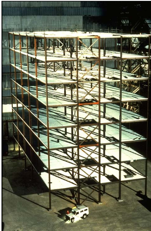
Figure 2.1 Cardington test building prior to concreting of the floors
