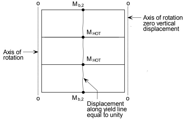
Figure 6.7 Yield line perpendicular to the unprotected beams edge condition on Sides A and C
