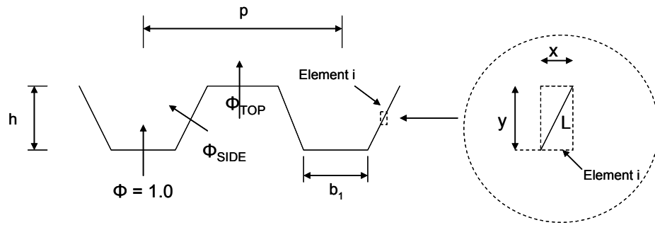
Figure 6.10 Configuration Factors for trapezoidal decks
