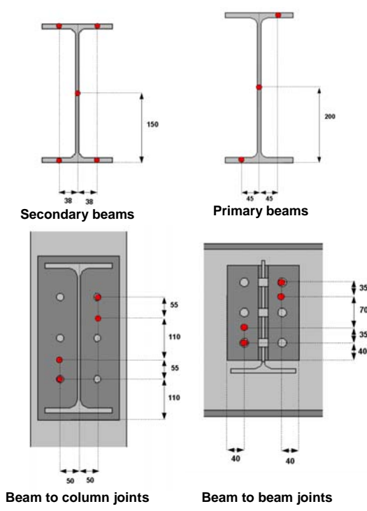
Figure 7.7 Location of thermocouples on each instrumented steelwork cross section
