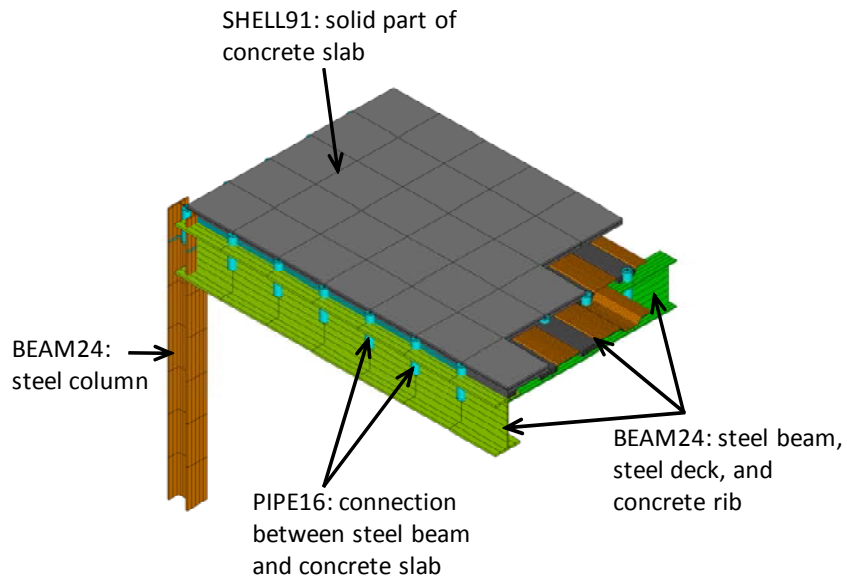
Figure 8.1 Detail of the structural modelling
