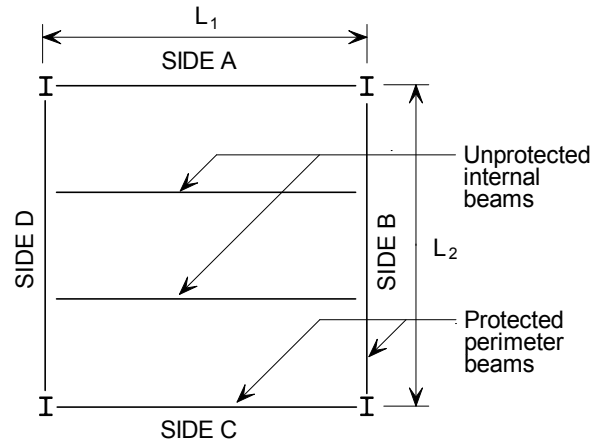
Figure 6.5 Typical floor design zone
