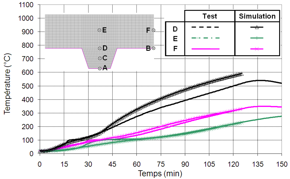
Figure 8.5 Temperature comparison between test and numerical calculation - composite slab
