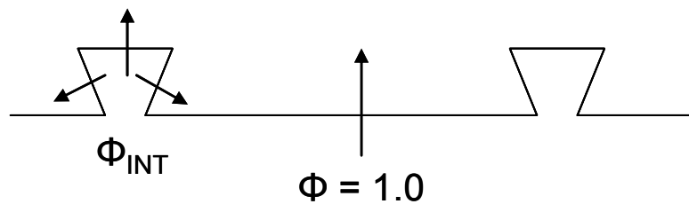
Figure 6.11 Configuration Factors for re-entrant decks
