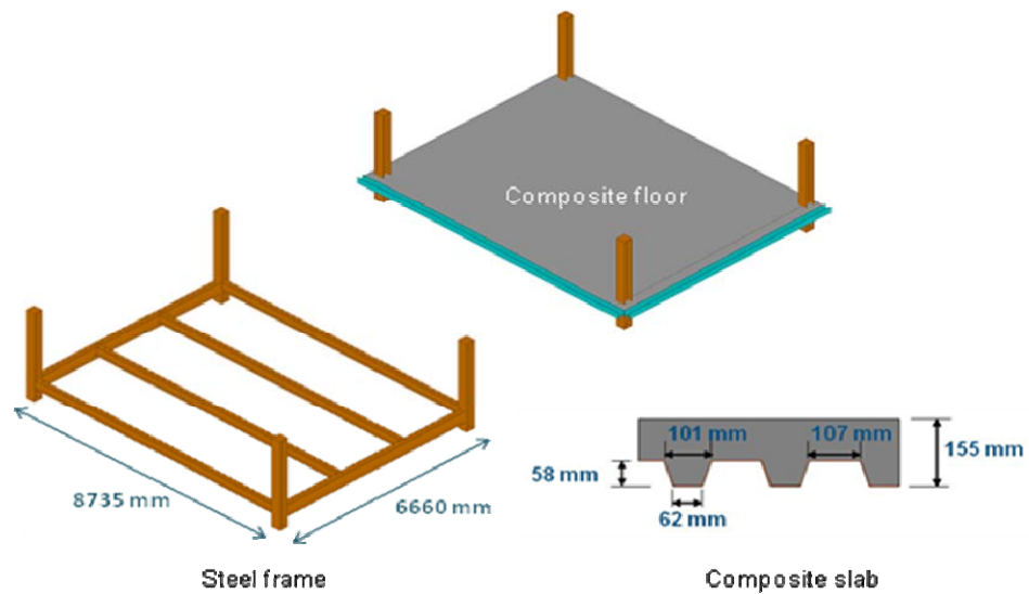
Figure 7.1 Fire test set-up
