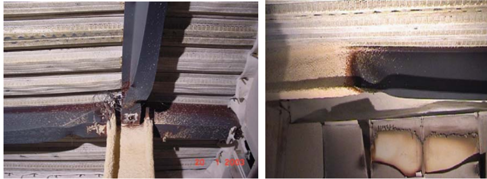
Figure 2.26 Various deformed steel beams
