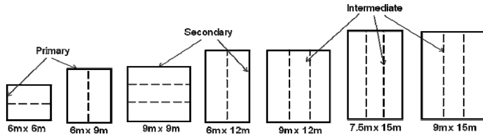
Figure 8.10 Floors considered in the parametric numerical study
