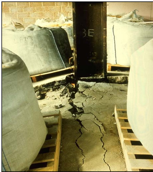
Figure 2.21 Cracked floor slab in region of non-overlapped mesh
