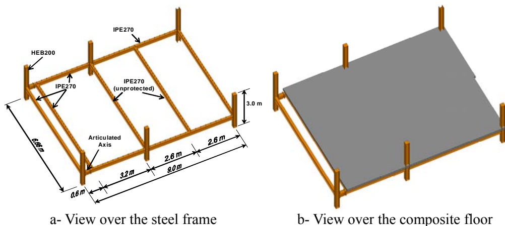
Figure 7.22 Fire test set-up
